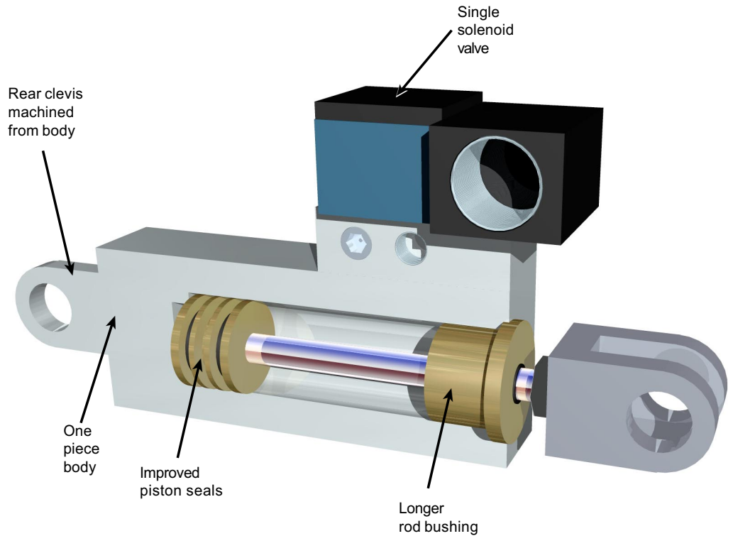
Cutaway of a Single Solenoid
